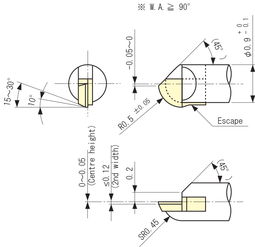
Cutting edge details (20:1)
