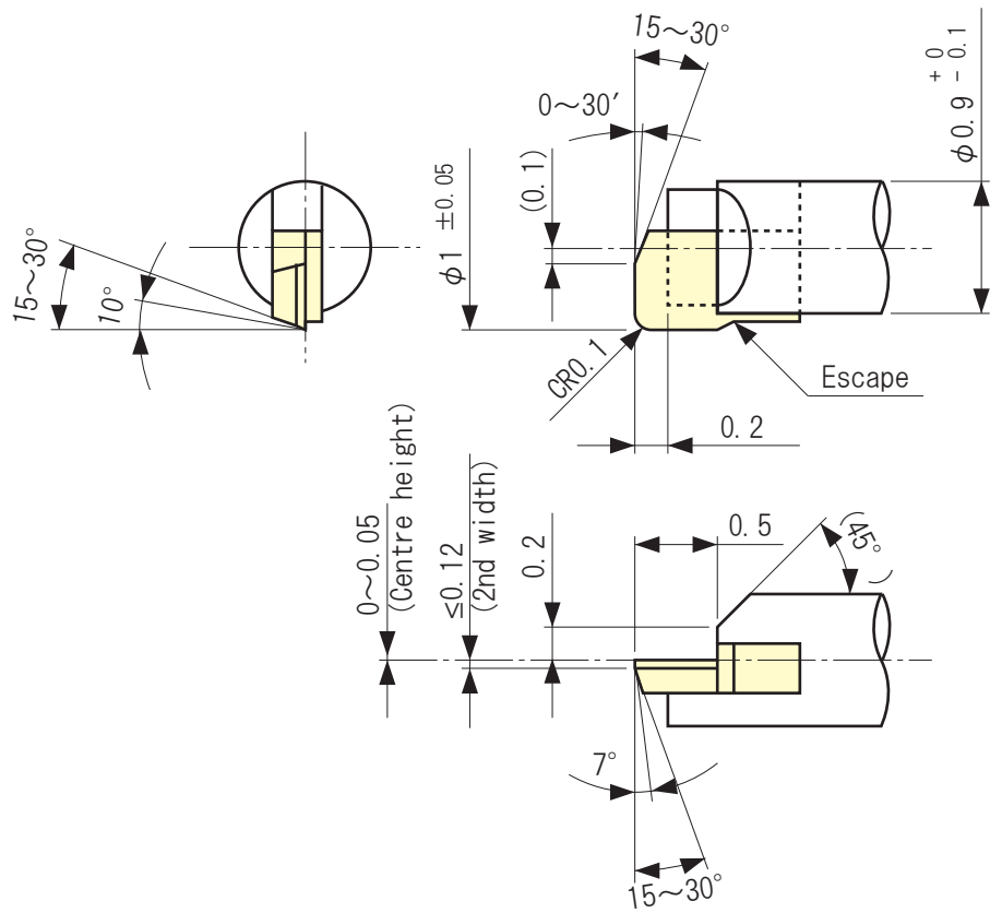
Cutting edge details (20:1)
